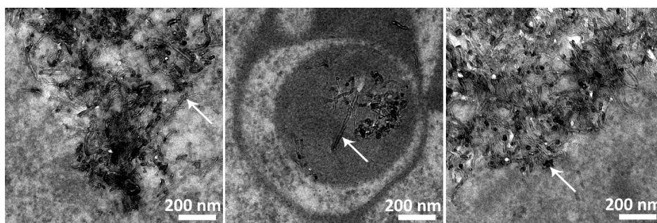
Figure 6. Different MWCNTs are located in different cellular compartments. Interior of alveolar M\phi recovered from BALF at 1 day postexposure to F-MWCNTs (A) and P-MWCNTs (B) by intratracheal instillation. P-MWCNTs at 21 days postexposure are shown on the right (C). Panels are TEM images of representative cells from rats exposed to a one-time bolus dose ( 200\ \mu\text{g} ) of MWCNTs suspended in dispersion media.
