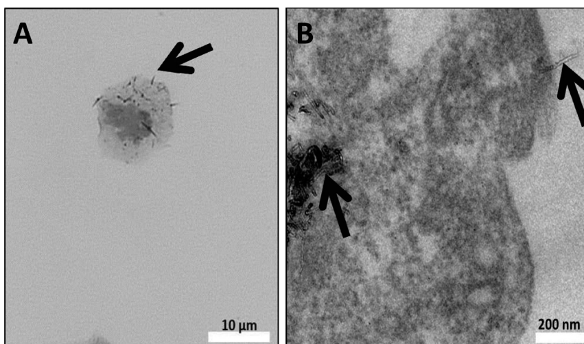
Figure 7. F-MWCNT uptake by M\phi . Cells recovered from BALF at 1 day postexposure to F-MWCNTs by intratracheal instillation. Bright-field image (A) of an alveolar macrophage with protruding F-MWCNTs (linear, black particles), verified by TEM (B), suggests cellular entry by penetration. BAL cells were stained with Diff Qwik for bright-field microscopy. Black arrows point to F-MWCNT.
